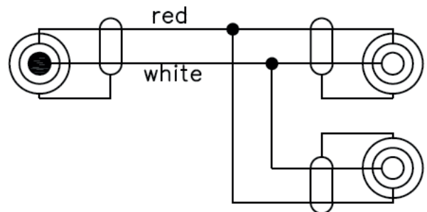
Wiring Layout
