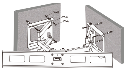
Fig. 13: Wall mounting
