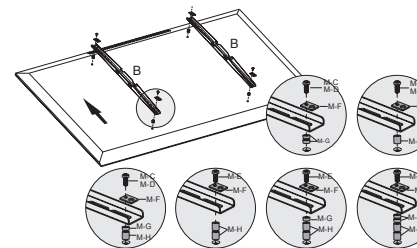
Fig. 17: Flat screens with arched back 2
