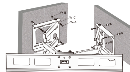
Fig.23: Montage mural
