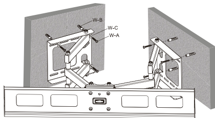
Fig. 3: Wandmontage
