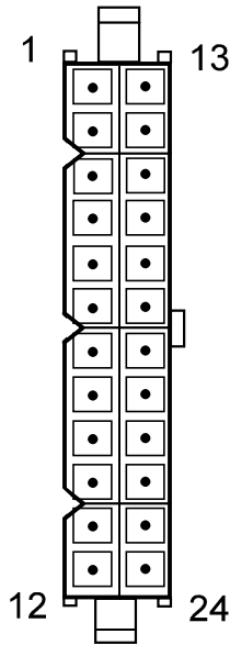
ATX 1.0 -jack 24 contacts
