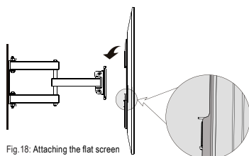
Fig.18: Attaching the flat screen
