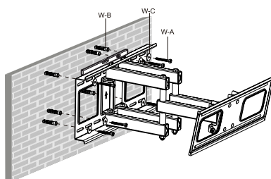
Fig. 13: Wall mounting
