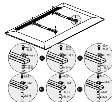
Fig. 16: Flat screens with arched back 1
