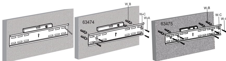
Fig. 1: Wandmontage
