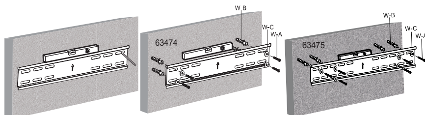
Fig.9: Montage mural
