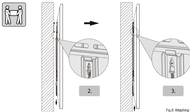
Fig. 8: Attaching the flat screen
