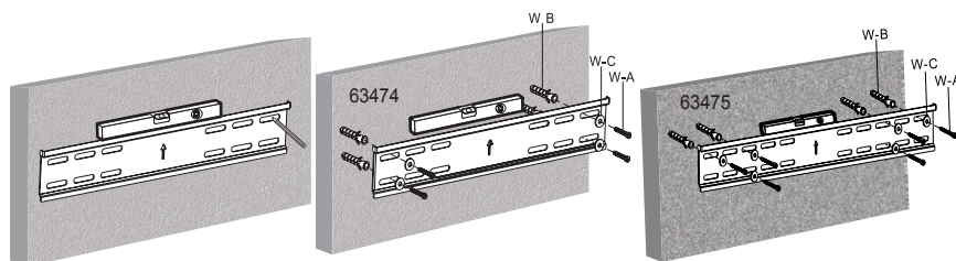
Fig. 5: Wall mounting
