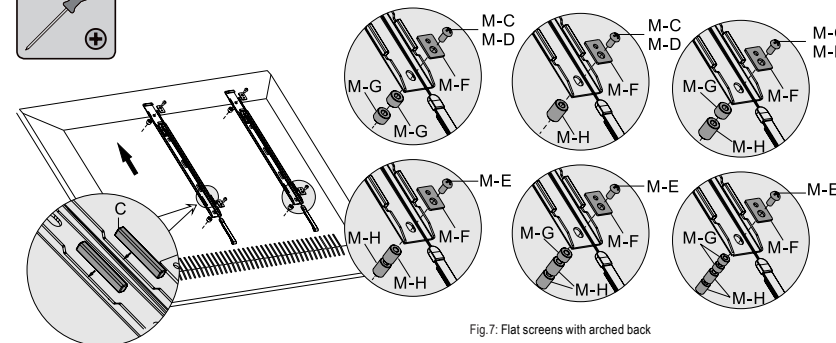
Fig. 7: Flat screens with arched back
