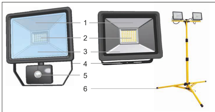
Fig.8: Product parts
