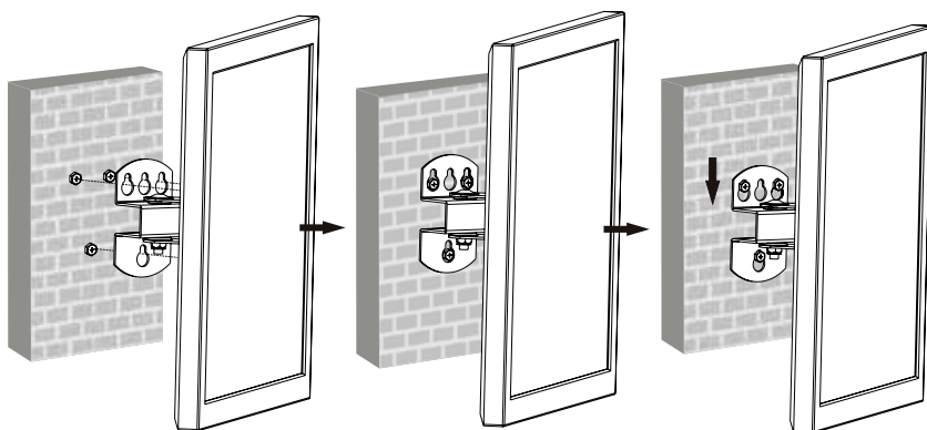
Fig. 11: Attaching and locking the flat screen
