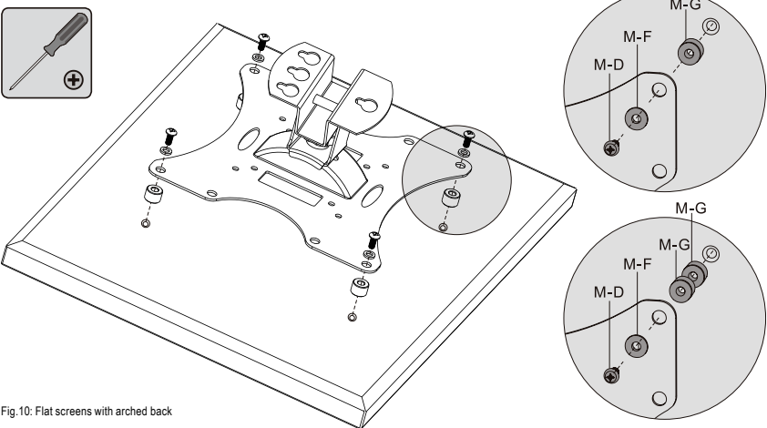
Fig.10: Flat screens with arched back
